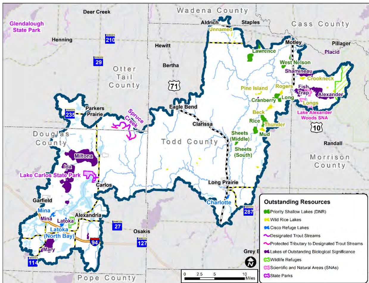
Figure 2.5. Outstanding resources and habitat in the Long Prairie River Watershed.
