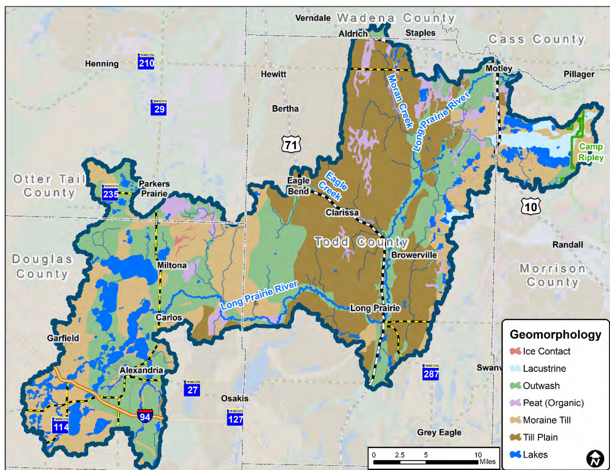
Figure 2.2. Geomorphology of the Long Prairie River Watershed.
